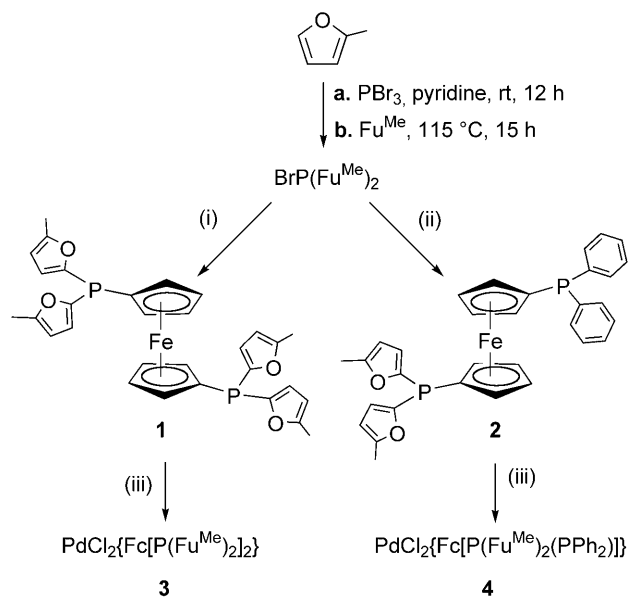
Scheme 1. Reagents and conditions: (i) 0.5 equivs. \text{FeCp}_2\text{Li}_2 -TMEDA, hexane, room temperature, 2 h; (ii) 1 equiv. \text{CpFe}(\text{Cp}(\text{PPh}_2))\text{Li} , THF, -50^\circ\text{C} , 12 h; (iii) 1 equiv. \text{PdCl}_2(\text{PhCN})_2 , \text{CH}_2\text{Cl}_2 , room temperature, 20 min.
